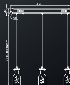
433 [REPLACEABLE WYMIENNY] 15W (79W), 1050 Lm, 4000K [LED] METAL + AKRYL / METAL + ACRYLIC
